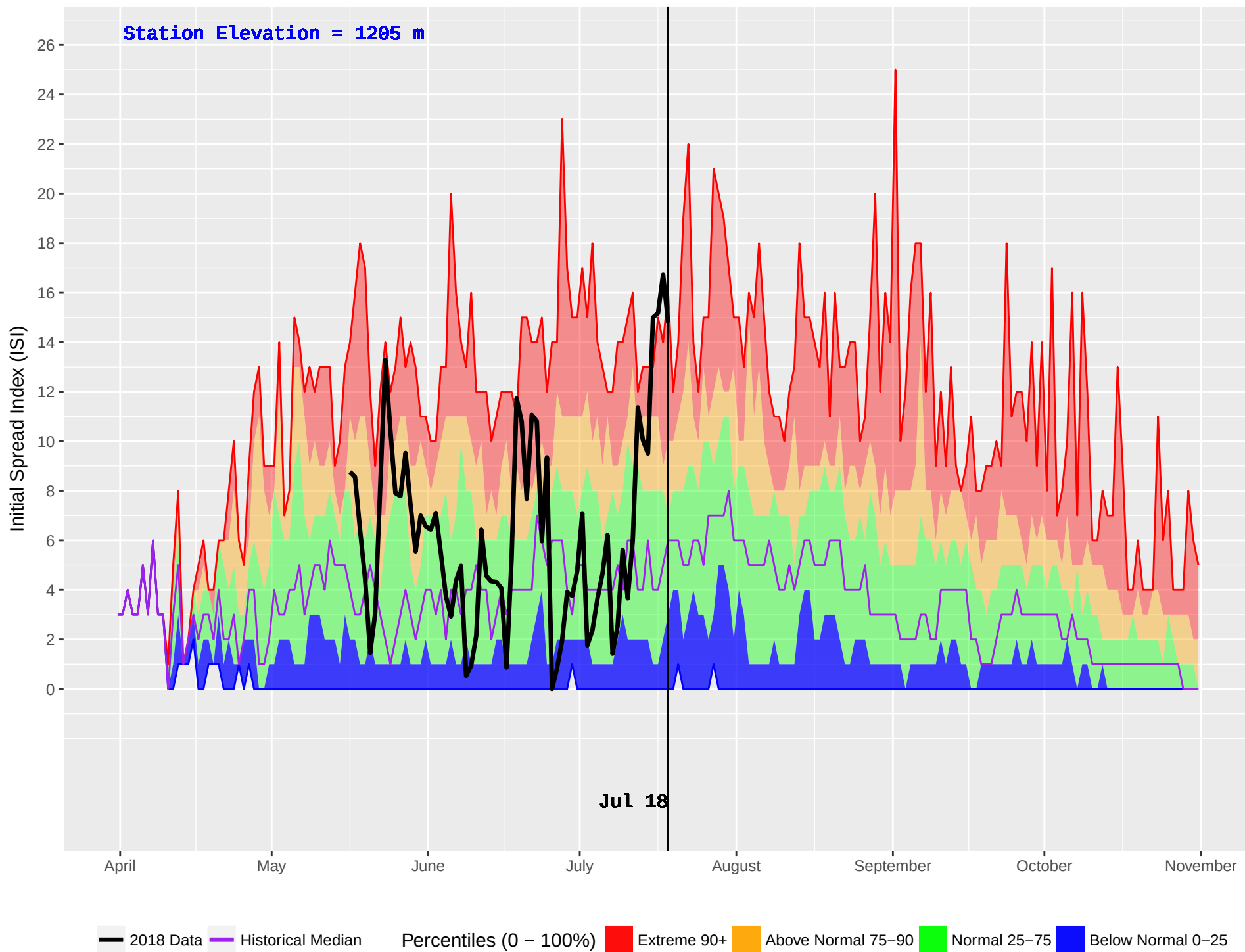
GWYNETH LAKE (309) : Historical (1986–2016) and Current (2018) Daily Initial Spread Index (ISI)
