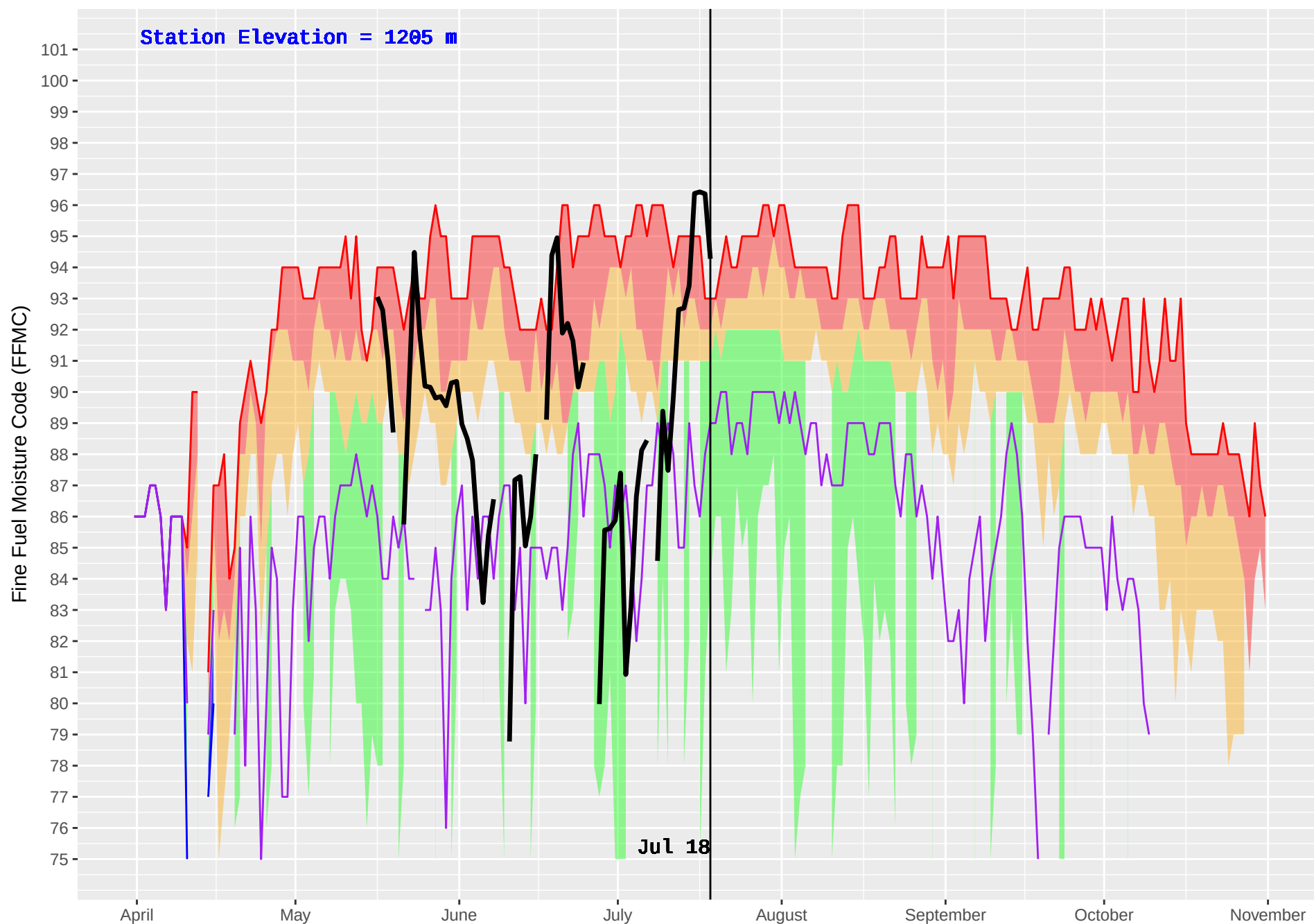
GWYNETH LAKE (309) : Historical (1986–2016) and Current (2018) Daily Fine Fuel Moisture Code (FFMC)
